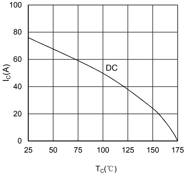
Figure 15. Collector Current vs Case temperature IGBT-inverter
