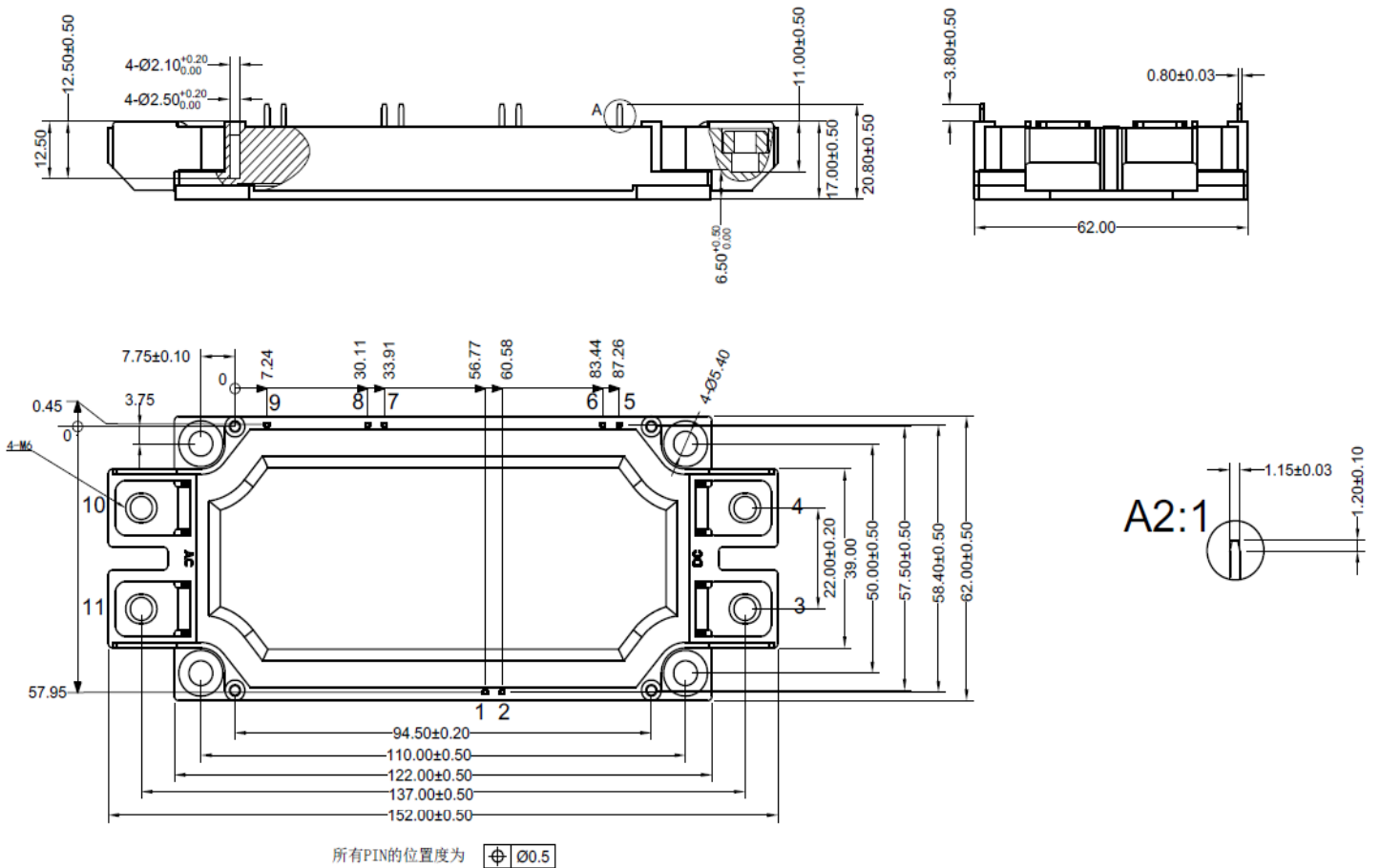
Figure 15. Package Outline
