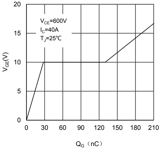
Figure 13. Gate Charge vs Gate Emitter Voltage
