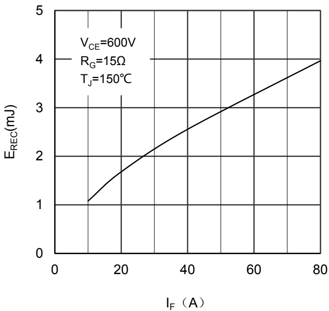
Figure 11. Switching Energy vs Forward Current Diode
